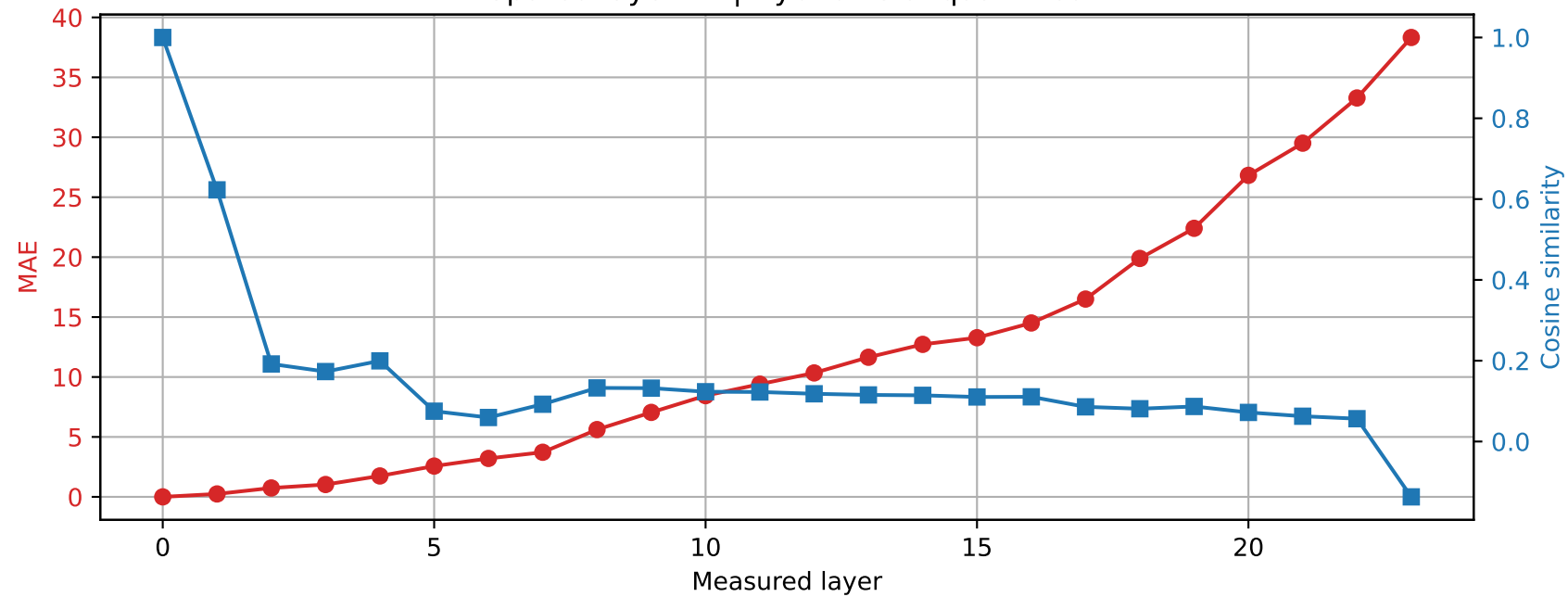
SmolLM2-1.7B-Instruct | Prompt 1 Spared layer 11 | Hybrid vs unquantized
