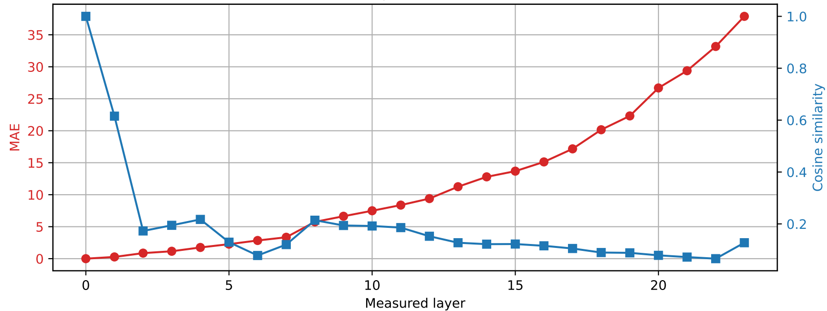
SmolLM2-1.7B-Instruct | Prompt 2 Spared layer 4 | Hybrid vs unquantized
