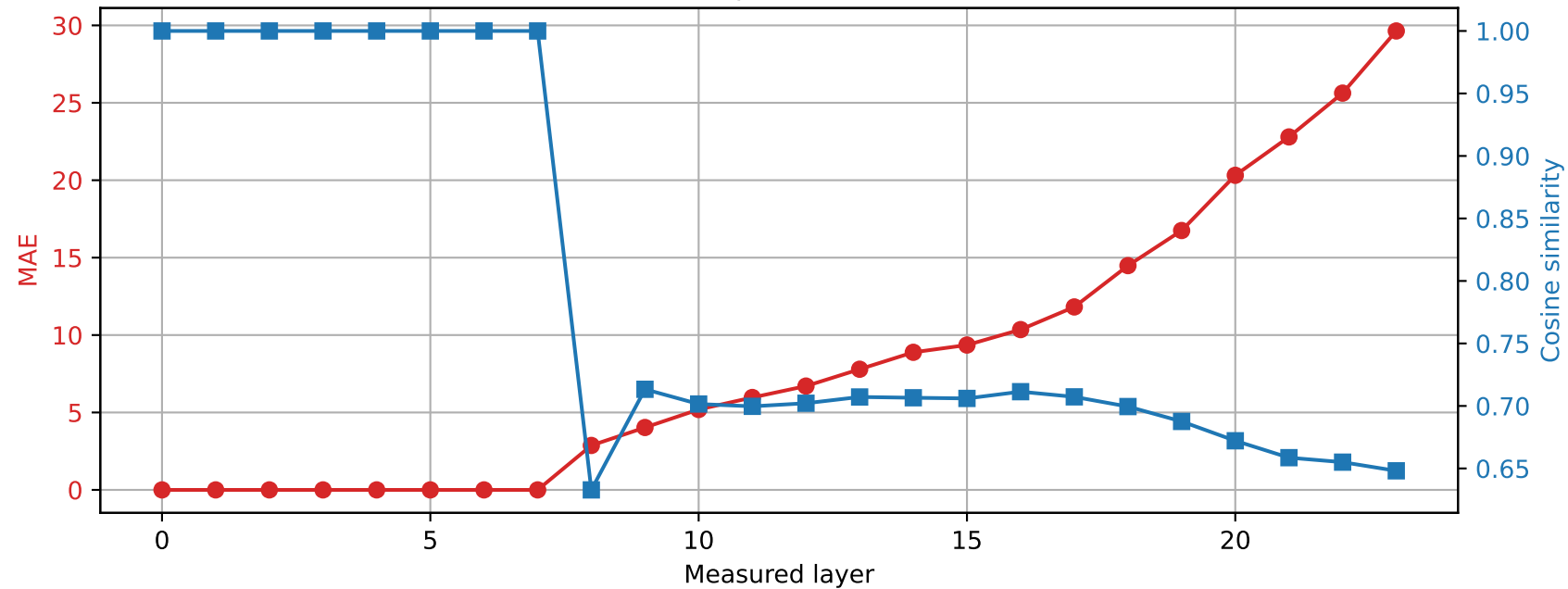
SmolLM2-1.7B-Instruct | Prompt 2 Spared layer 7 | Hybrid vs quantized
