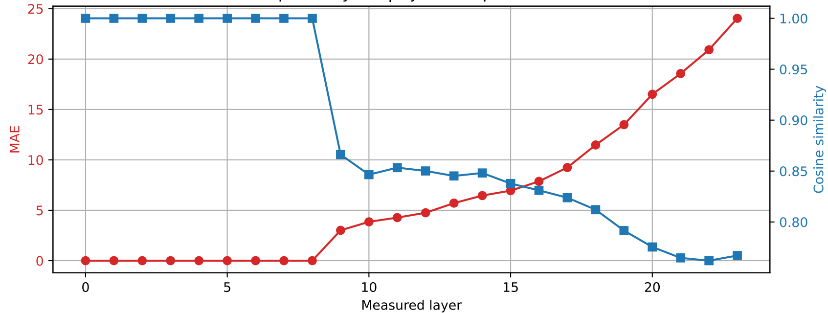
SmolLM2-1.7B-Instruct | Prompt 2 Spared layer 8 | Hybrid vs quantized
