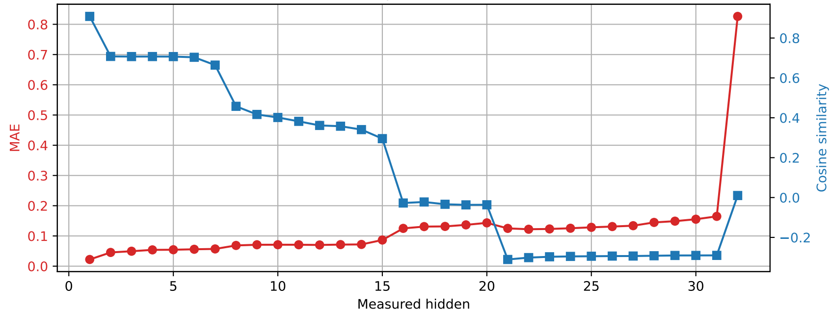
OLMo-7B-hf | Prompt 2 Spared layer 10 | Unquantized vs hybrid
