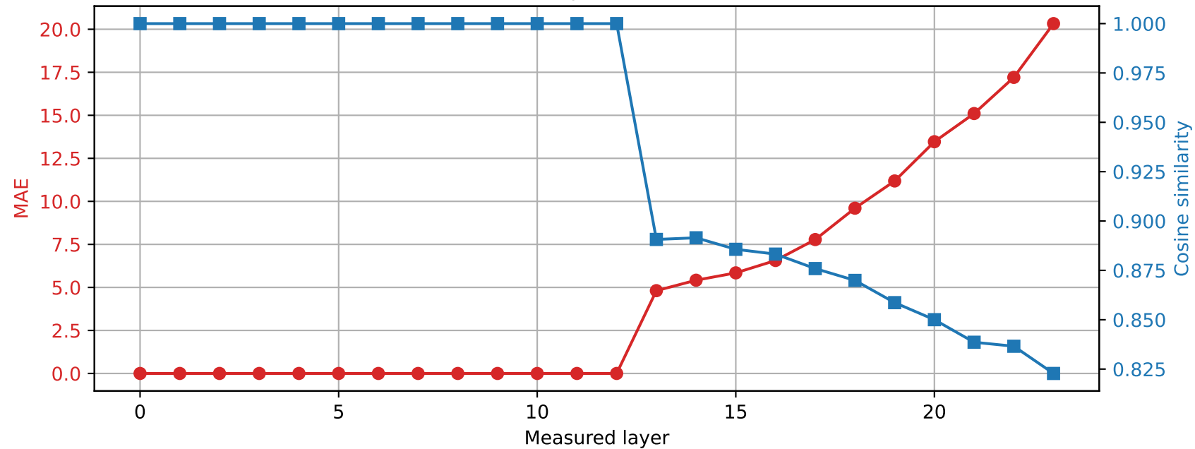
SmolLM2-1.7B-Instruct | Prompt 2 Spared layer 12 | Hybrid vs quantized
