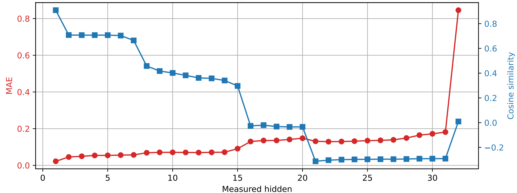
OLMo-7B-hf | Prompt 2 Spared layer 14 | Unquantized vs hybrid
