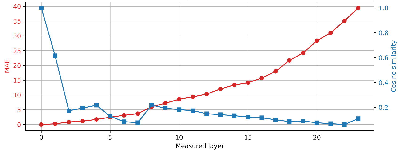
SmolLM2-1.7B-Instruct | Prompt 2 Spared layer 21 | Hybrid vs unquantized
