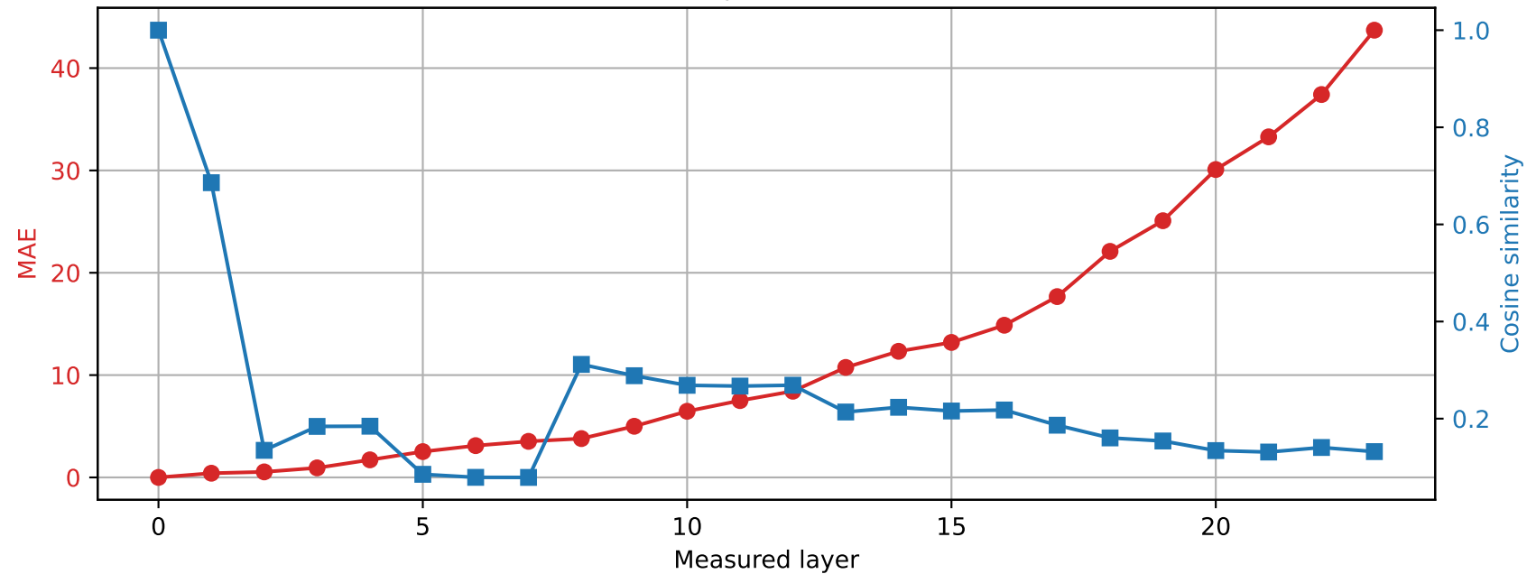
SmolLM2-1.7B-Instruct | Prompt 3 Spared layer 0 | Hybrid vs quantized
