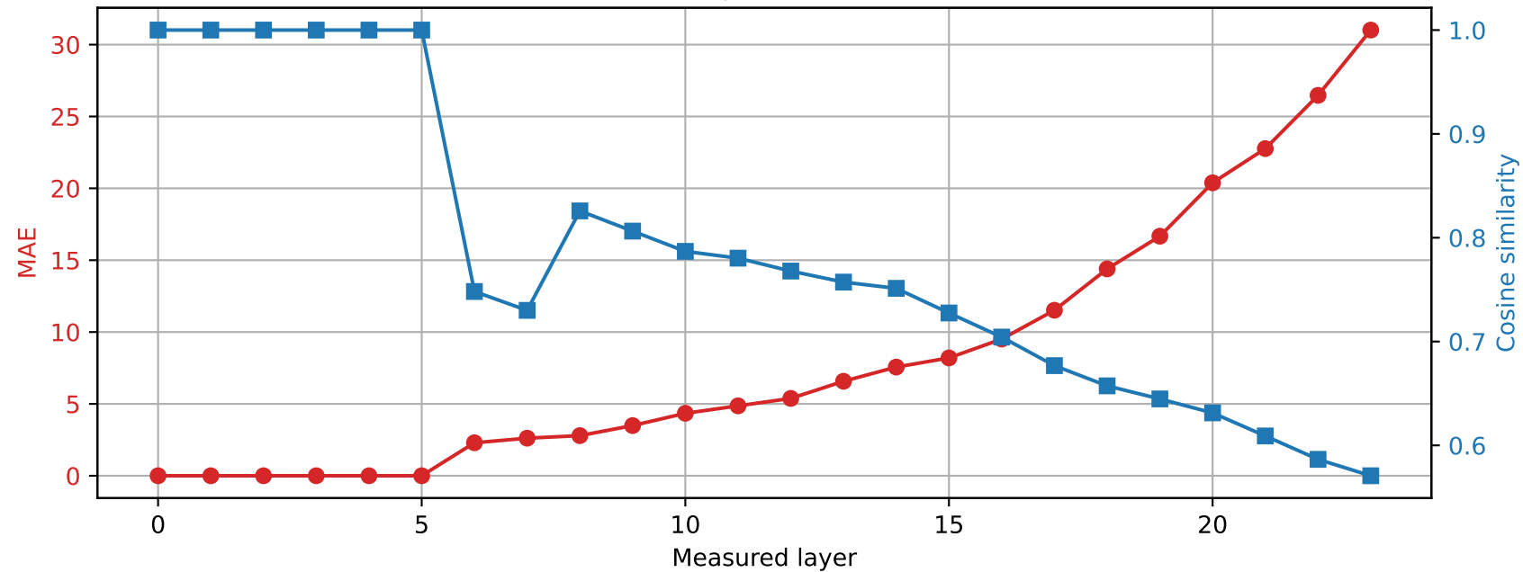
SmolLM2-1.7B-Instruct | Prompt 3 Spared layer 5 | Hybrid vs quantized
