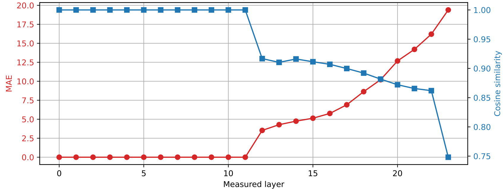
SmolLM2-1.7B-Instruct | Prompt 3 Spared layer 11 | Hybrid vs quantized
