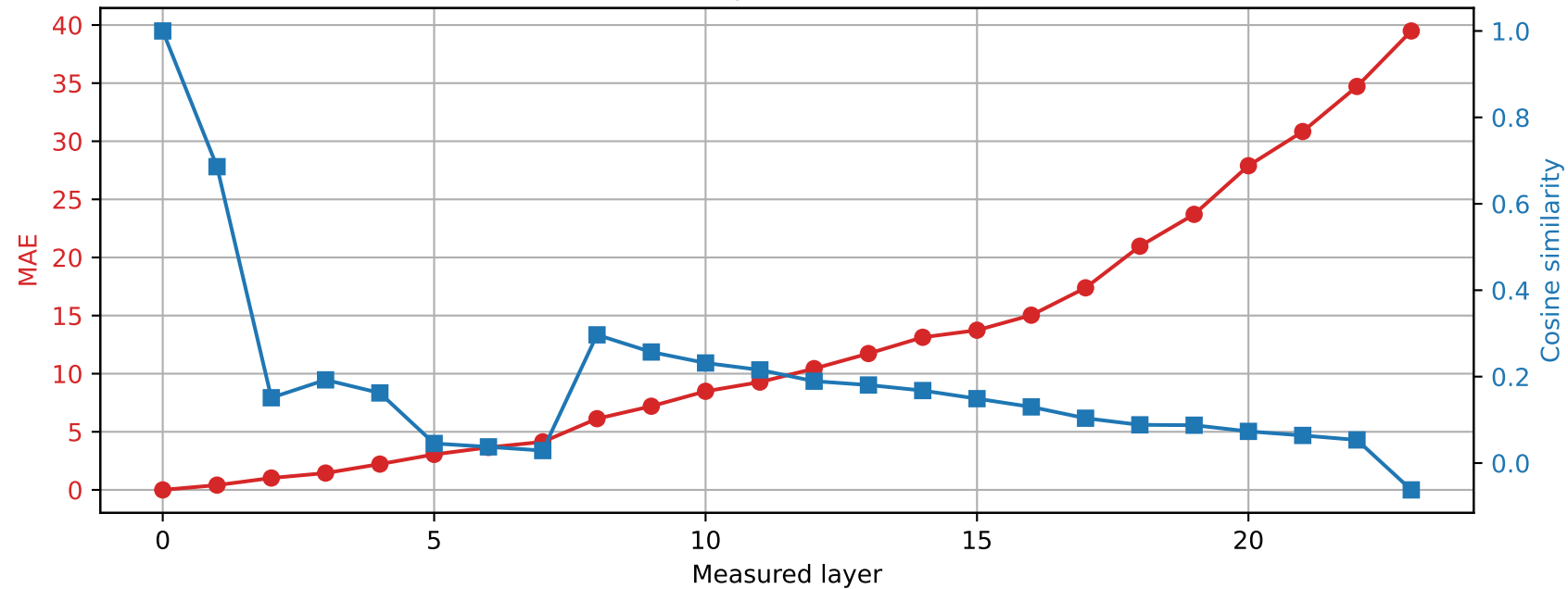
SmolLM2-1.7B-Instruct | Prompt 3 Spared layer 11 | Hybrid vs unquantized
