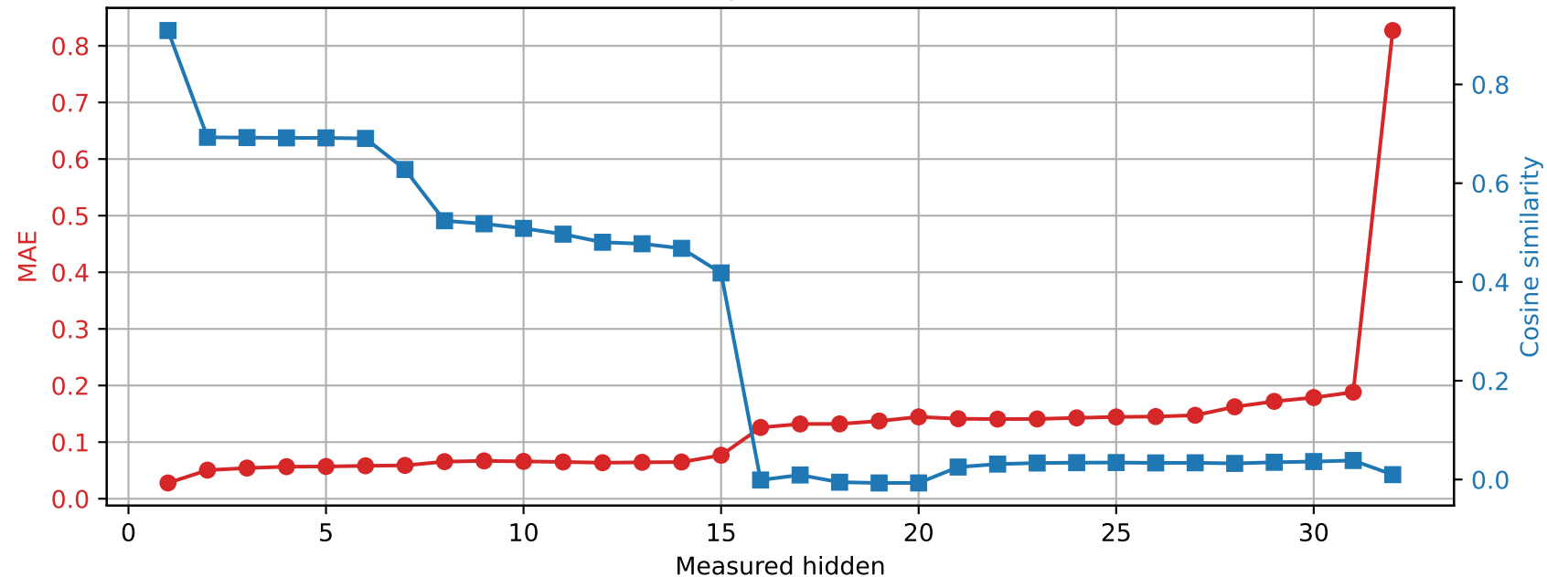
OLMo-7B-hf | Prompt 3 Spared layer 15 | Unquantized vs hybrid
