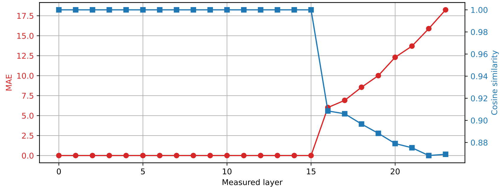
SmolLM2-1.7B-Instruct | Prompt 3 Spared layer 15 | Hybrid vs quantized
