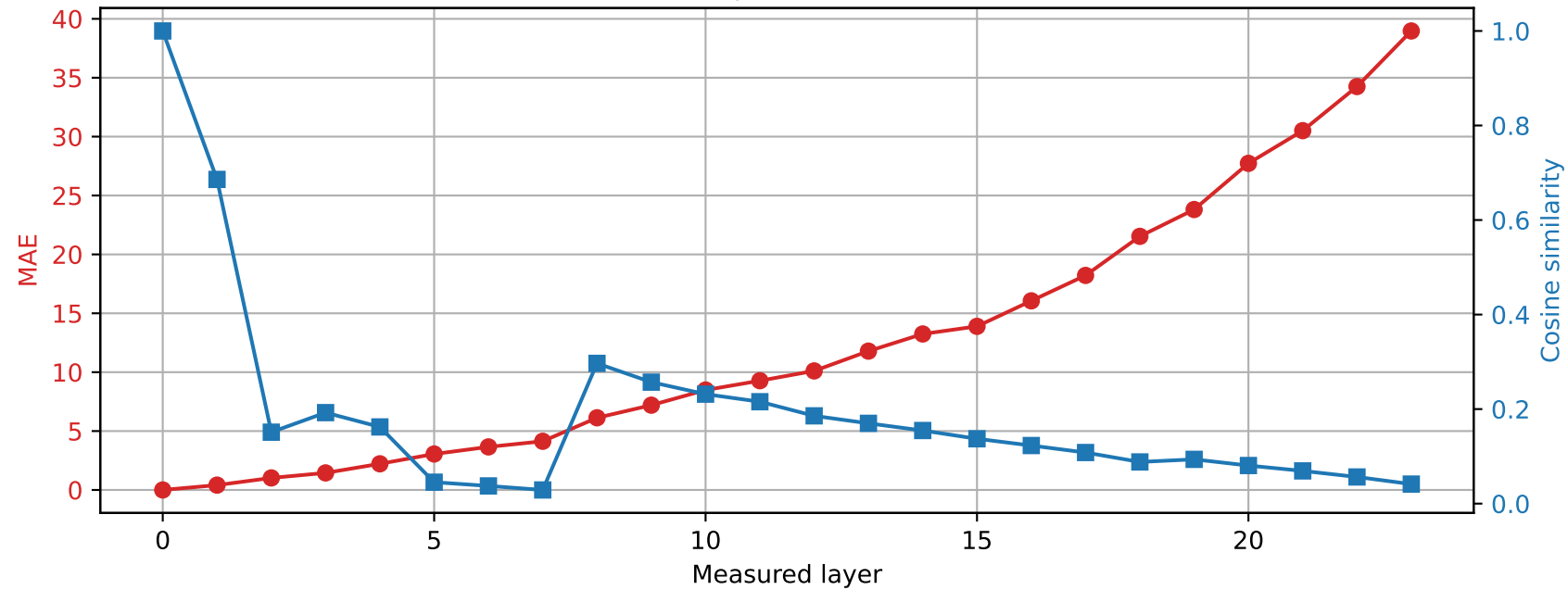
SmolLM2-1.7B-Instruct | Prompt 3 Spared layer 15 | Hybrid vs unquantized
