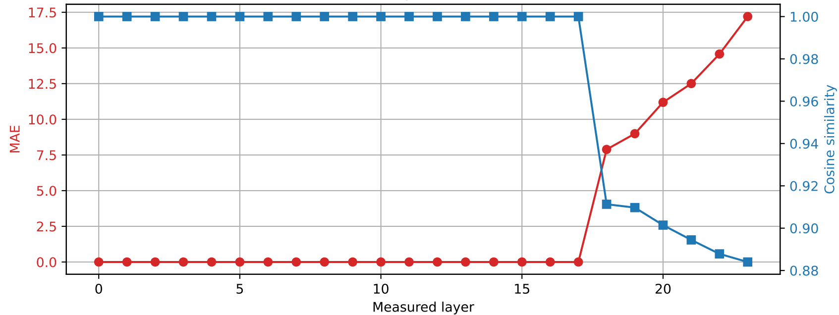
SmolLM2-1.7B-Instruct | Prompt 3 Spared layer 17 | Hybrid vs quantized
