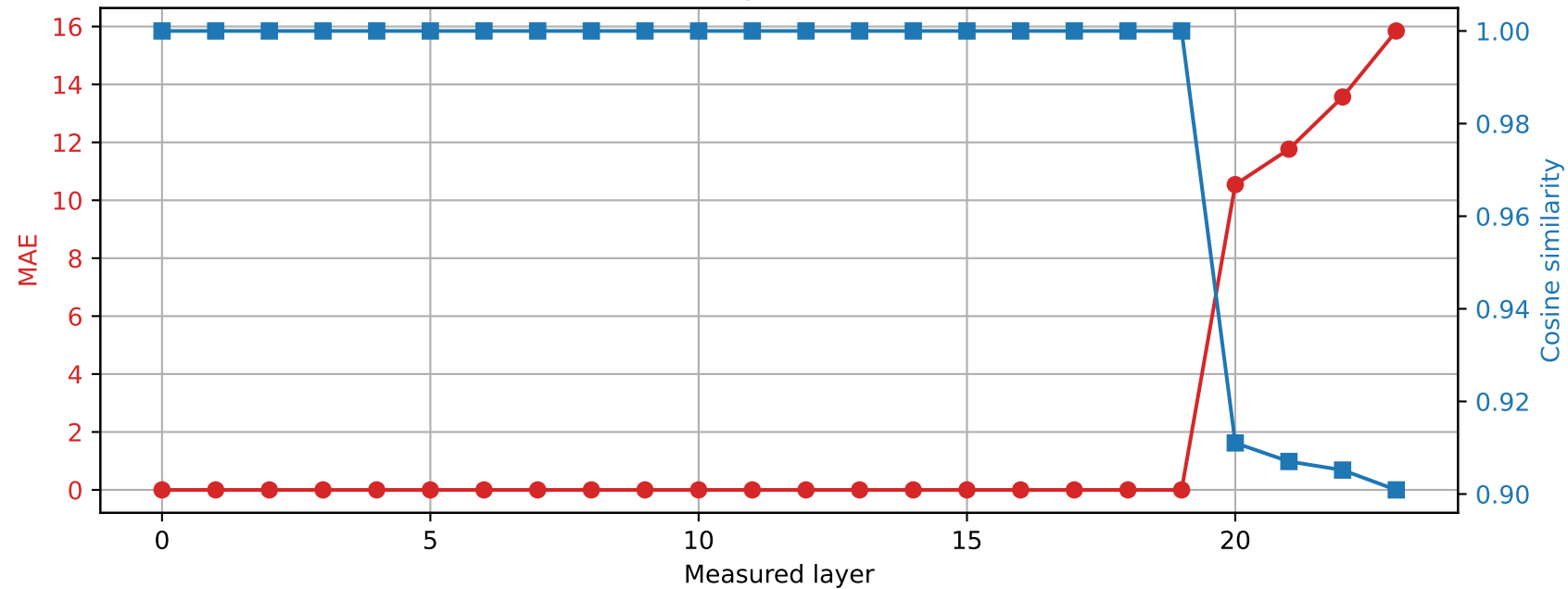
SmolLM2-1.7B-Instruct | Prompt 3 Spared layer 19 | Hybrid vs quantized
