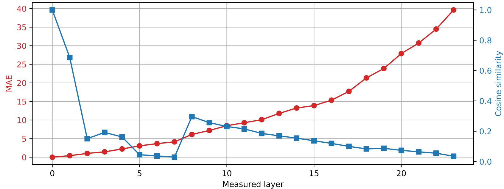
SmolLM2-1.7B-Instruct | Prompt 3 Spared layer 22 | Hybrid vs unquantized
