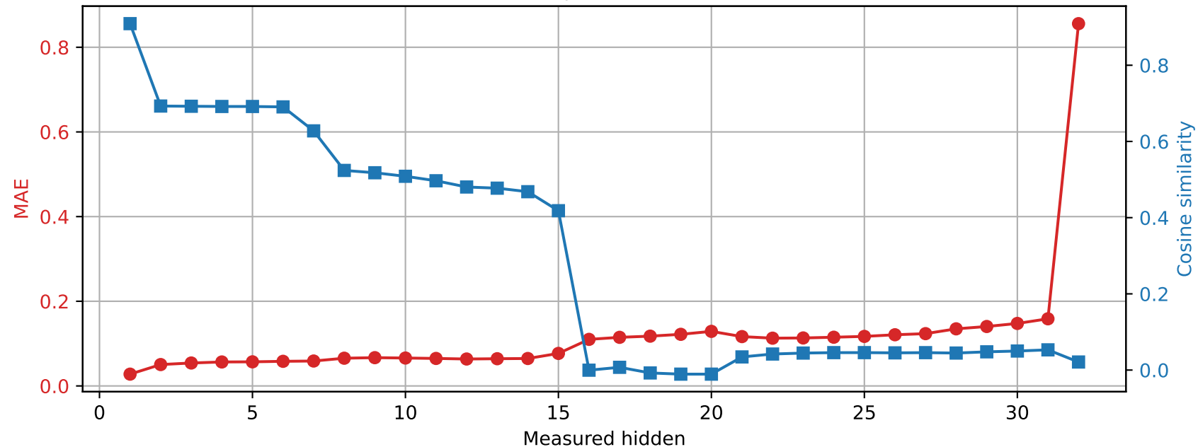
OLMo-7B-hf | Prompt 3 Spared layer 24 | Unquantized vs hybrid
