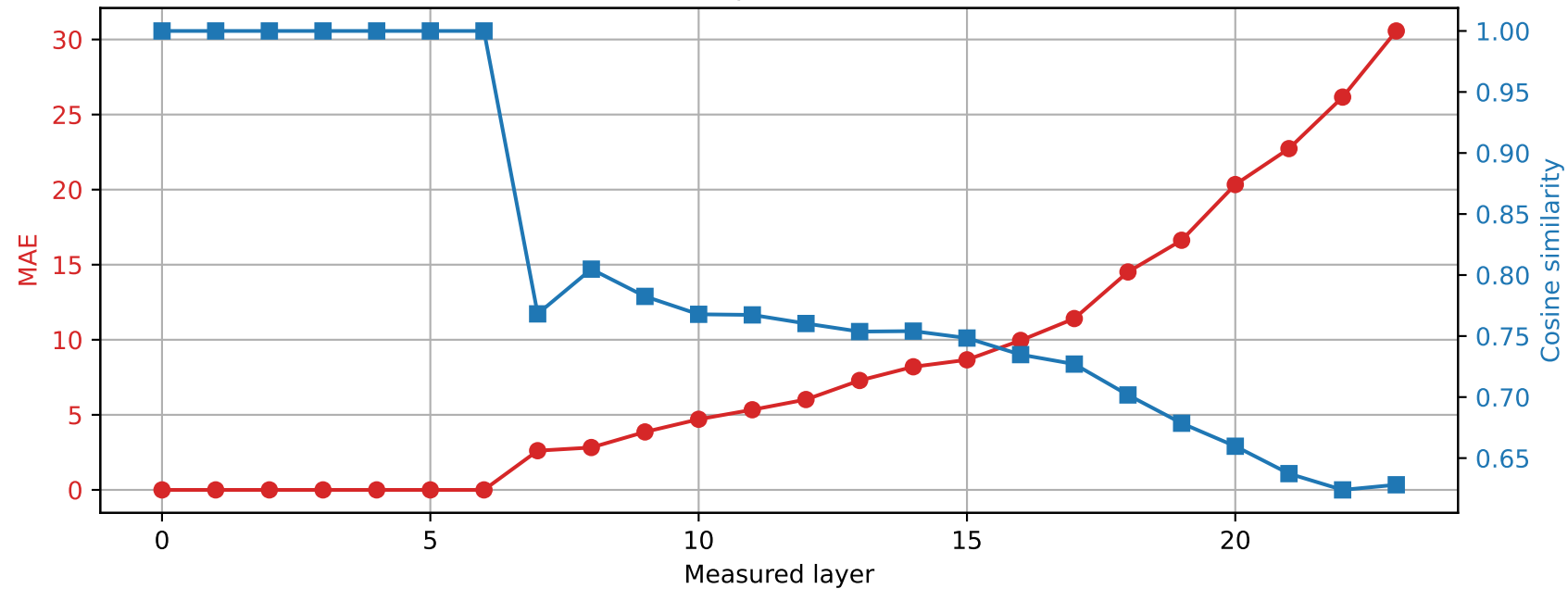
SmolLM2-1.7B-Instruct | Prompt 4 Spared layer 6 | Hybrid vs quantized
