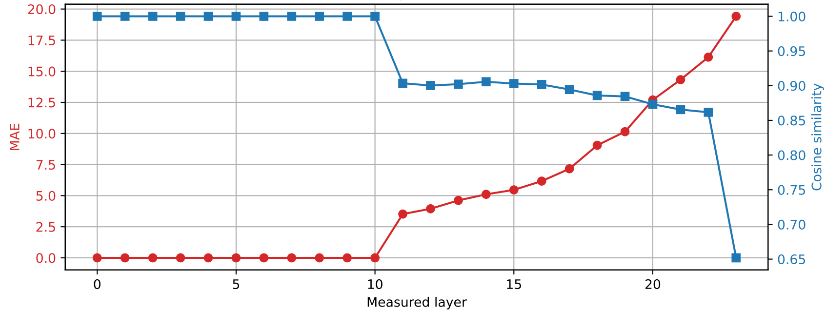
SmolLM2-1.7B-Instruct | Prompt 4 Spared layer 10 | Hybrid vs quantized
