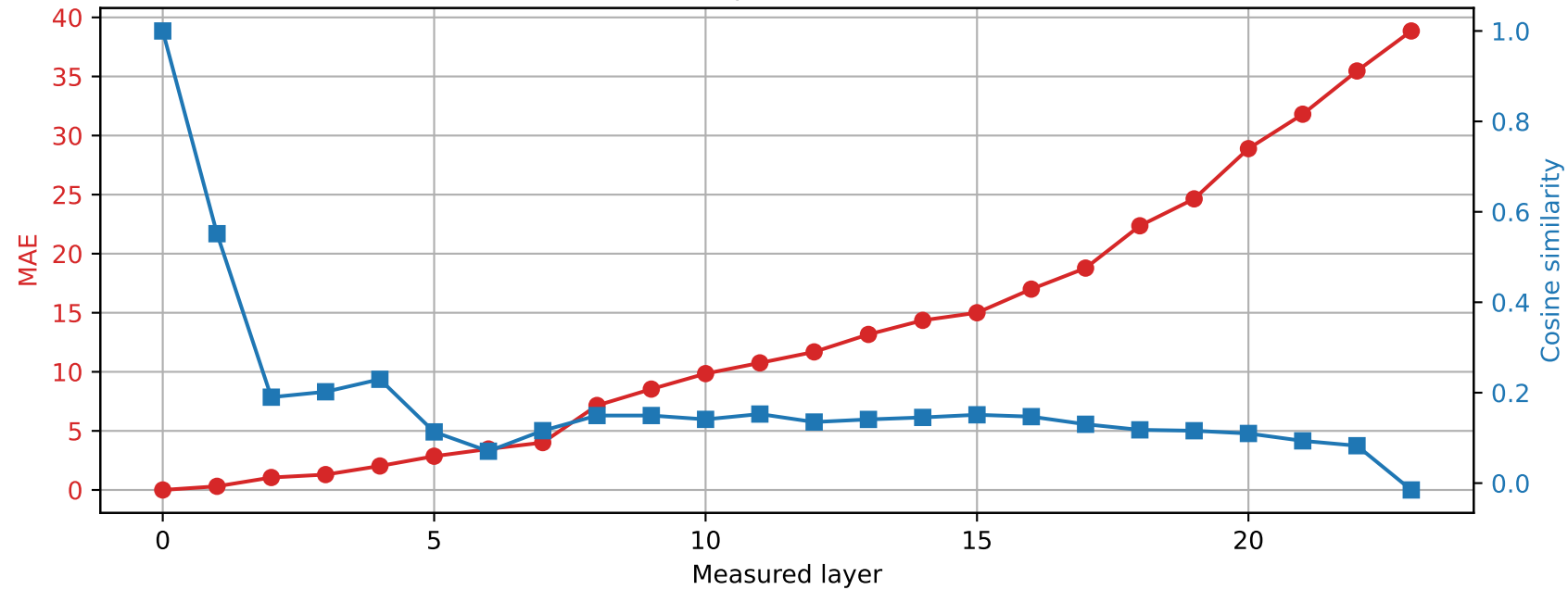
SmolLM2-1.7B-Instruct | Prompt 4 Spared layer 15 | Hybrid vs unquantized
