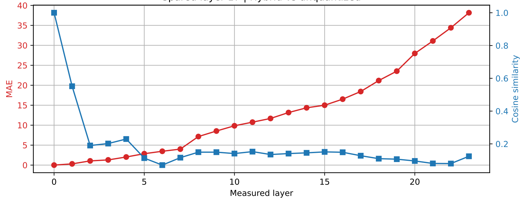
SmolLM2-1.7B-Instruct | Prompt 4 Spared layer 17 | Hybrid vs unquantized
