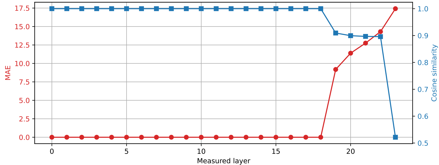
SmolLM2-1.7B-Instruct | Prompt 4 Spared layer 18 | Hybrid vs quantized
