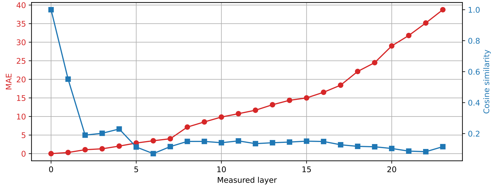
SmolLM2-1.7B-Instruct | Prompt 4 Spared layer 20 | Hybrid vs unquantized
