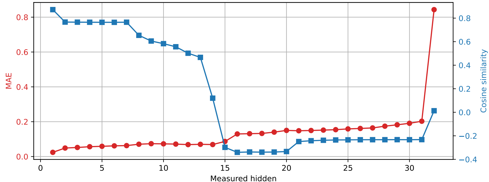
OLMo-7B-hf | Prompt 4 Spared layer 27 | Unquantized vs hybrid
