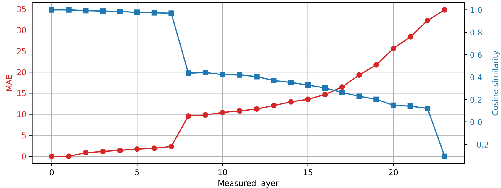
SmolLM2-1.7B-Instruct | Prompt 0 Spared layer 0 | Hybrid vs unquantized
