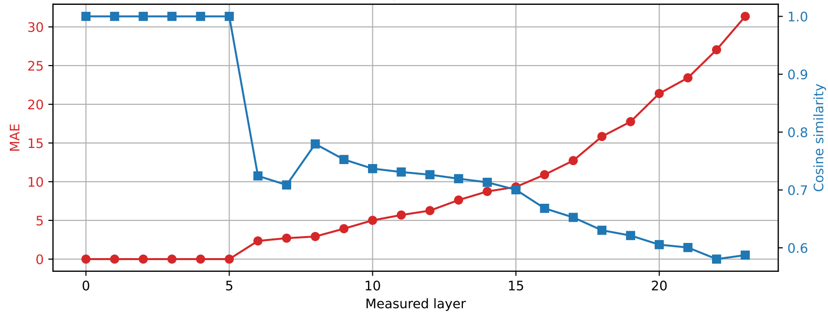
SmolLM2-1.7B-Instruct | Prompt 0 Spared layer 5 | Hybrid vs quantized
