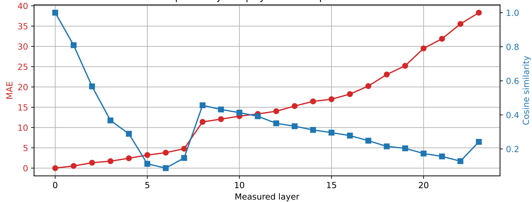
SmolLM2-1.7B-Instruct | Prompt 0 Spared layer 6 | Hybrid vs unquantized
