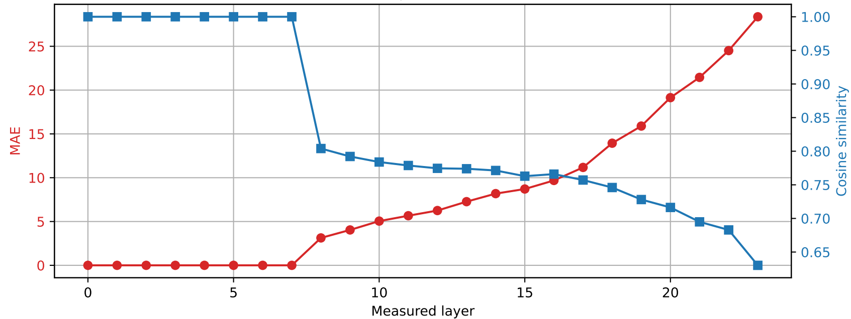
SmolLM2-1.7B-Instruct | Prompt 0 Spared layer 7 | Hybrid vs quantized
