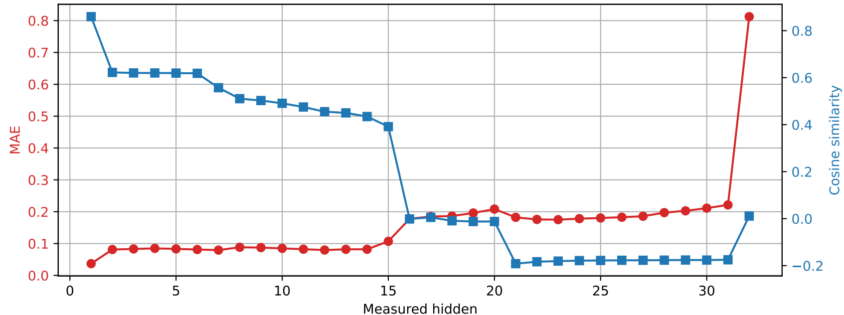
OLMo-7B-hf | Prompt 0 Spared layer 11 | Unquantized vs hybrid
