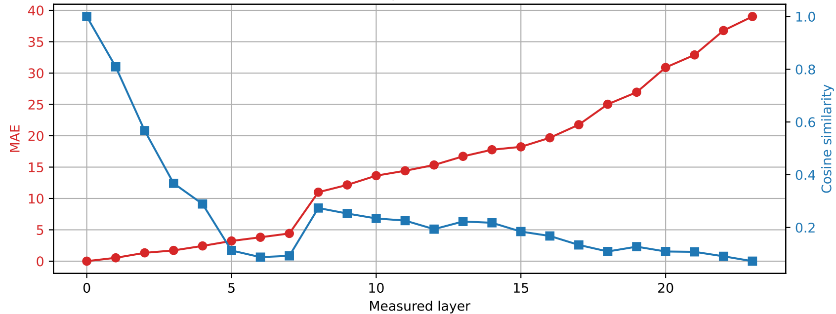
SmolLM2-1.7B-Instruct | Prompt 0 Spared layer 12 | Hybrid vs unquantized
