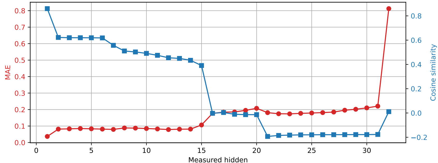
OLMo-7B-hf | Prompt 0 Spared layer 25 | Unquantized vs hybrid
