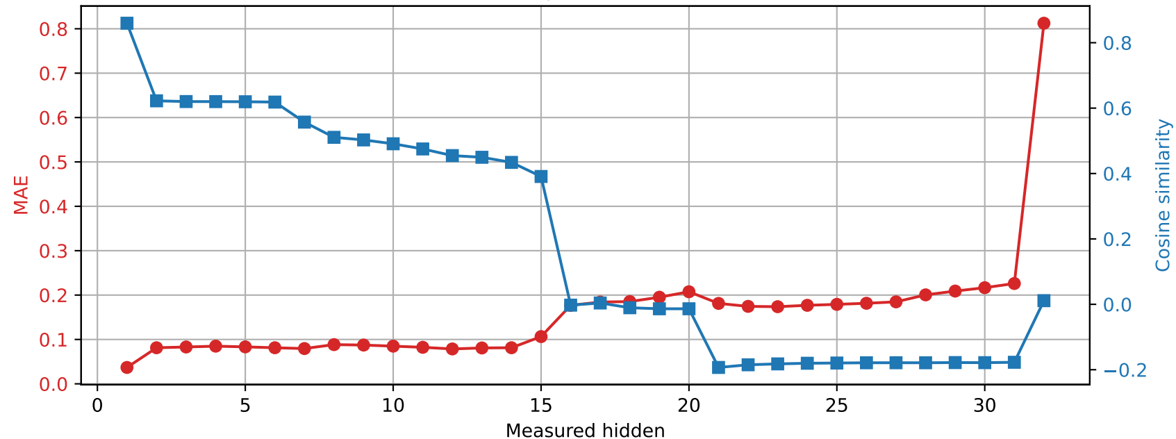
OLMo-7B-hf | Prompt 0 Spared layer 27 | Unquantized vs hybrid
