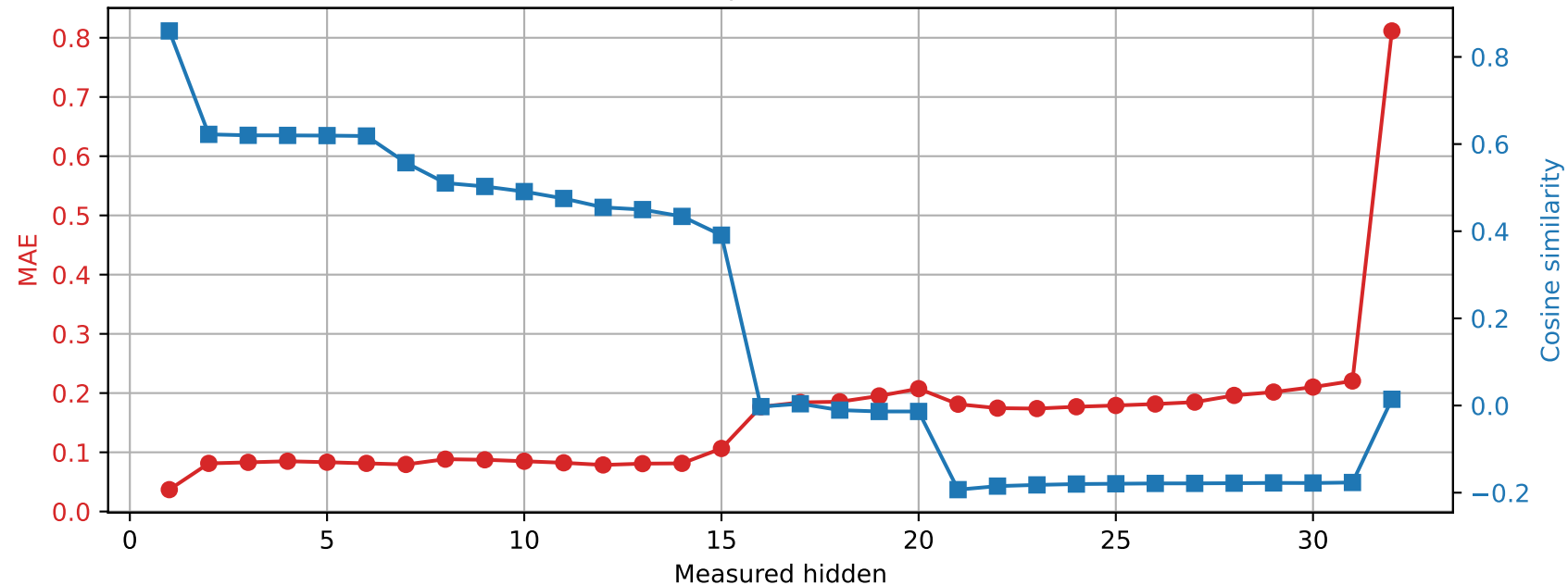
OLMo-7B-hf | Prompt 0 Spared layer 31 | Unquantized vs hybrid
