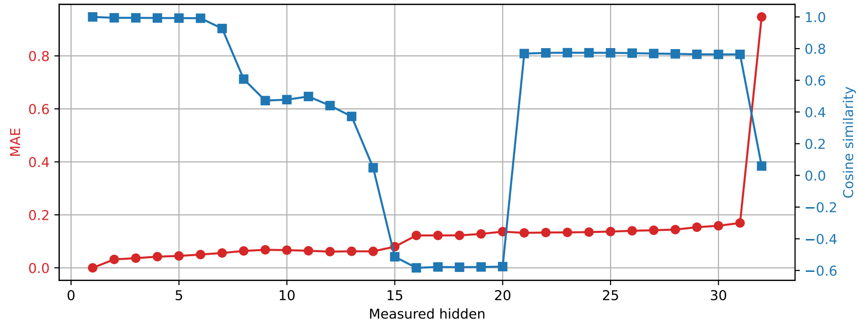
OLMo-7B-hf | Prompt 1 Spared layer 0 | Unquantized vs hybrid
