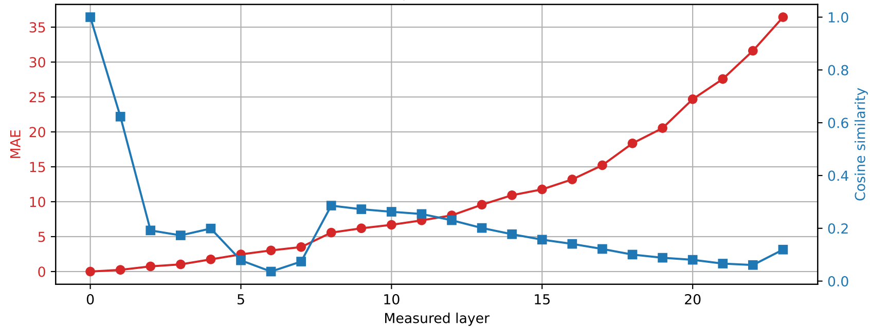
SmolLM2-1.7B-Instruct | Prompt 1 Spared layer 4 | Hybrid vs unquantized
