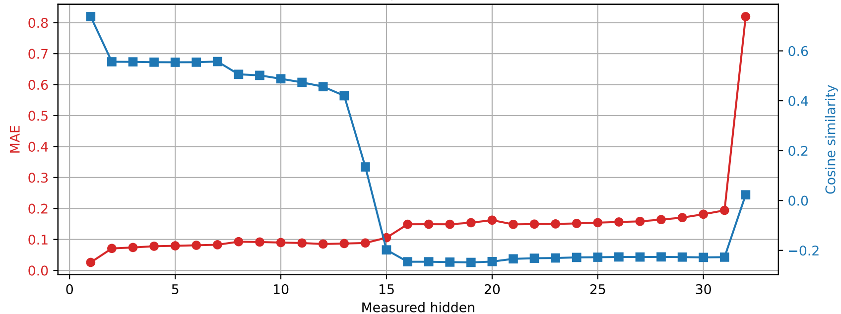
OLMo-7B-hf | Prompt 1 Spared layer 13 | Unquantized vs hybrid
