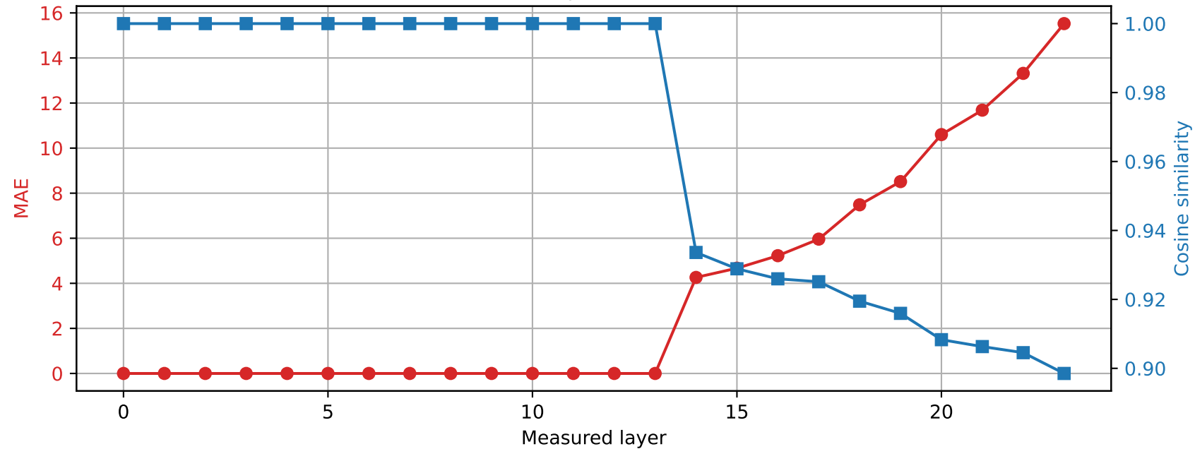
SmolLM2-1.7B-Instruct | Prompt 1 Spared layer 13 | Hybrid vs quantized
