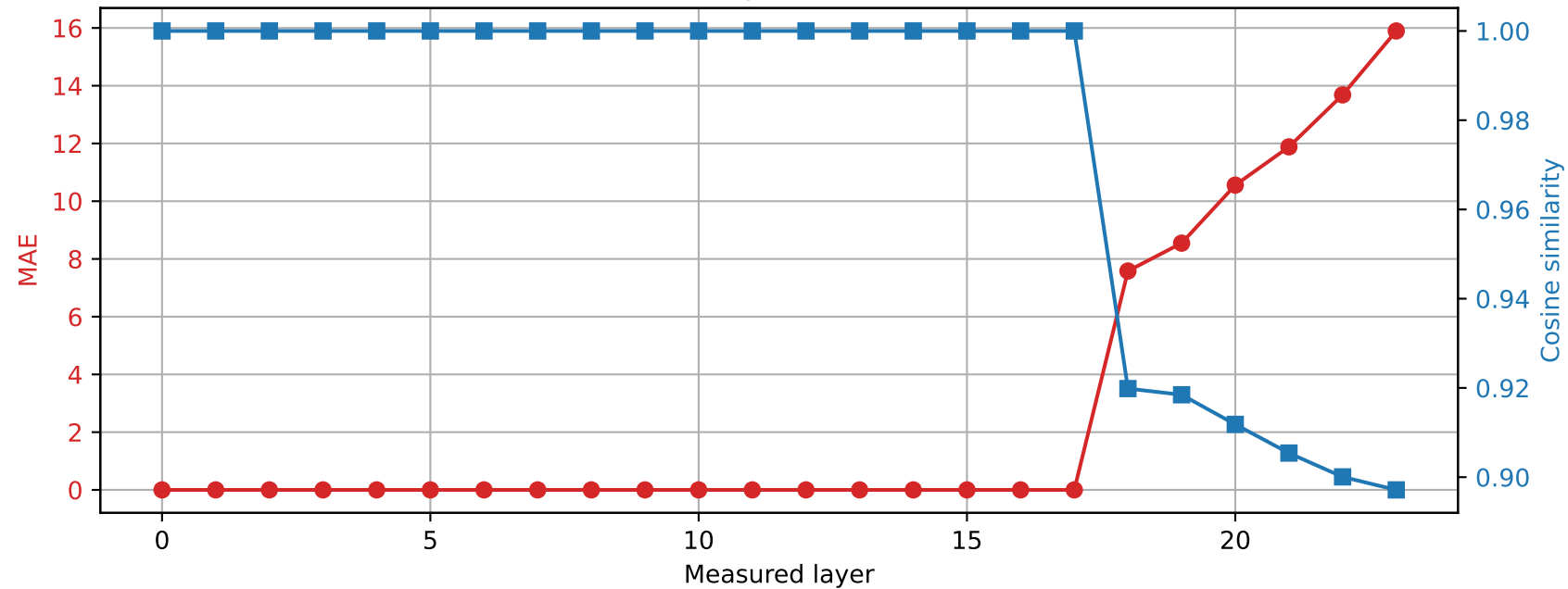
SmolLM2-1.7B-Instruct | Prompt 1 Spared layer 17 | Hybrid vs quantized
