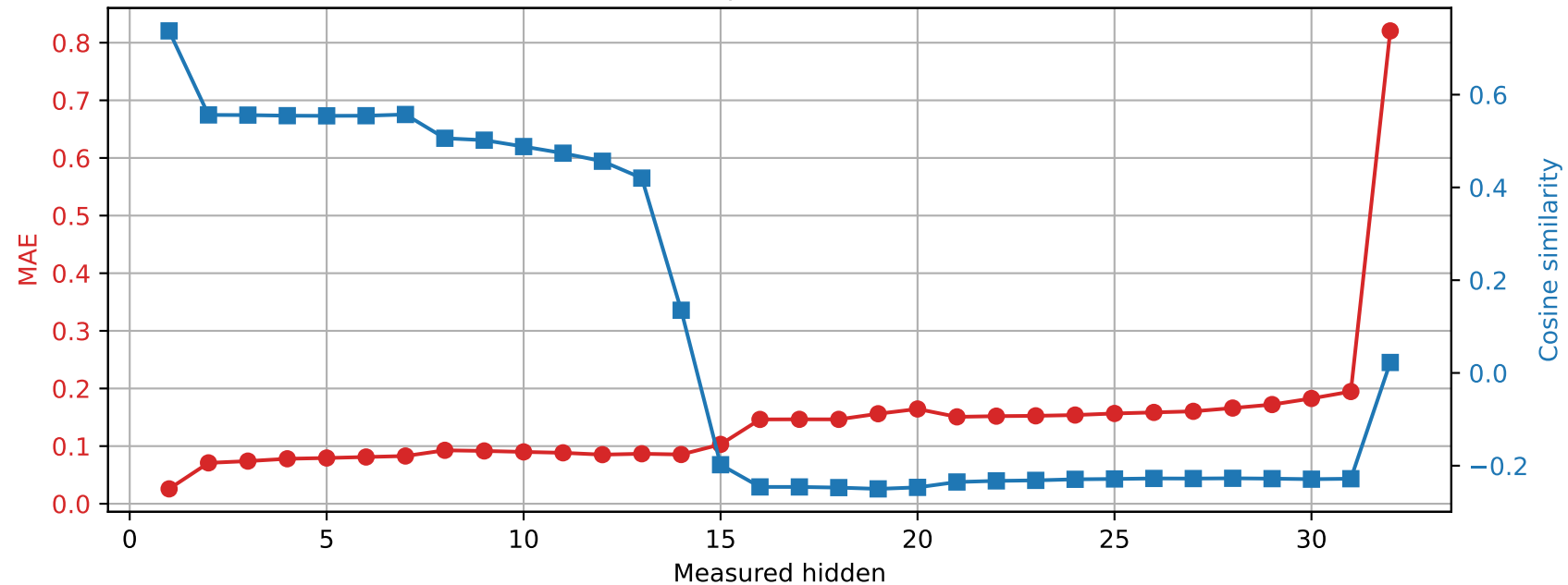
OLMo-7B-hf | Prompt 1 Spared layer 18 | Unquantized vs hybrid
