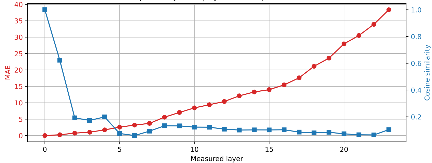
SmolLM2-1.7B-Instruct | Prompt 1 Spared layer 21 | Hybrid vs unquantized
