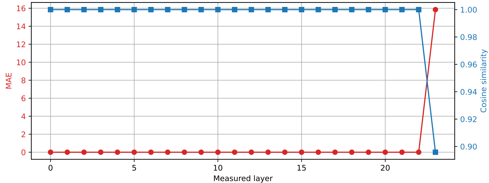
SmolLM2-1.7B-Instruct | Prompt 1 Spared layer 22 | Hybrid vs quantized
