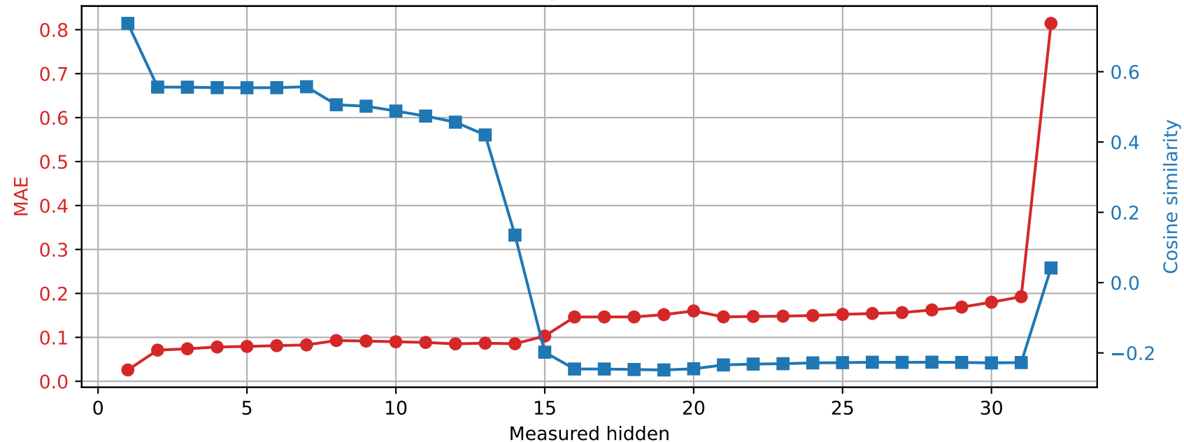
OLMo-7B-hf | Prompt 1 Spared layer 31 | Unquantized vs hybrid
