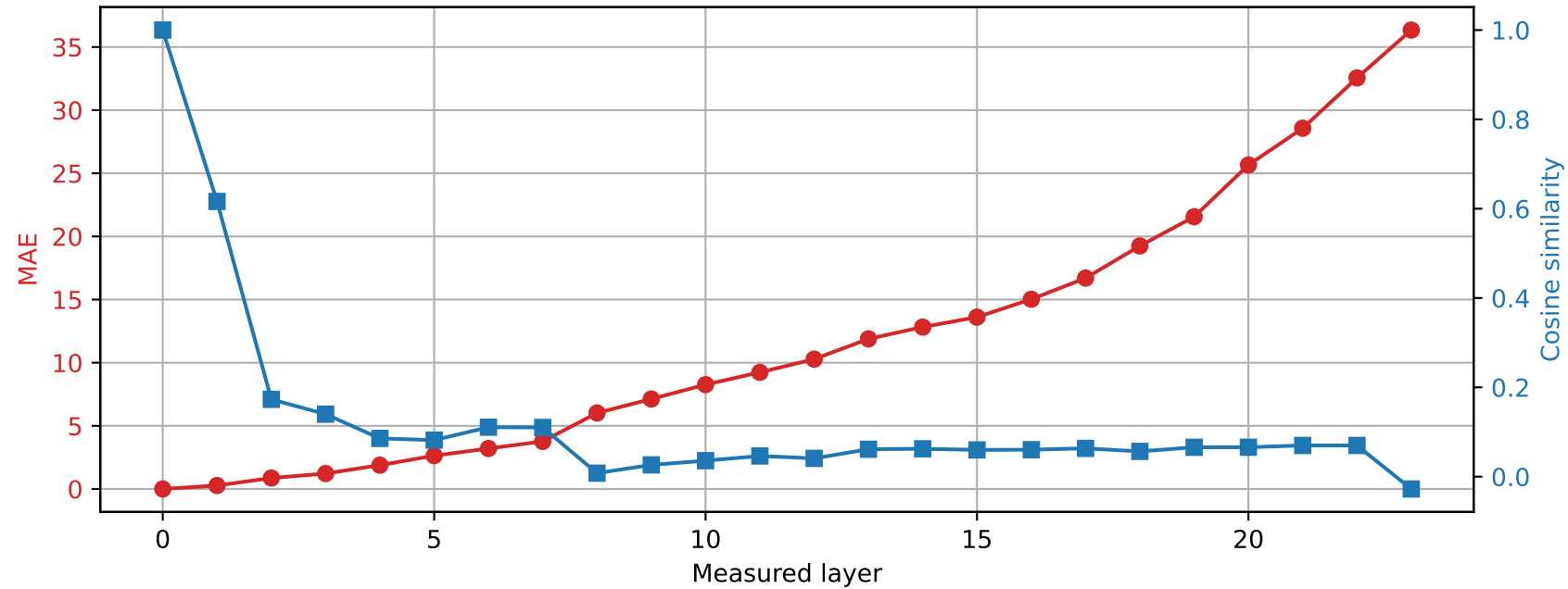
SmolLM2-1.7B-Instruct | Prompt 2 Spared layer 2 | Hybrid vs unquantized
