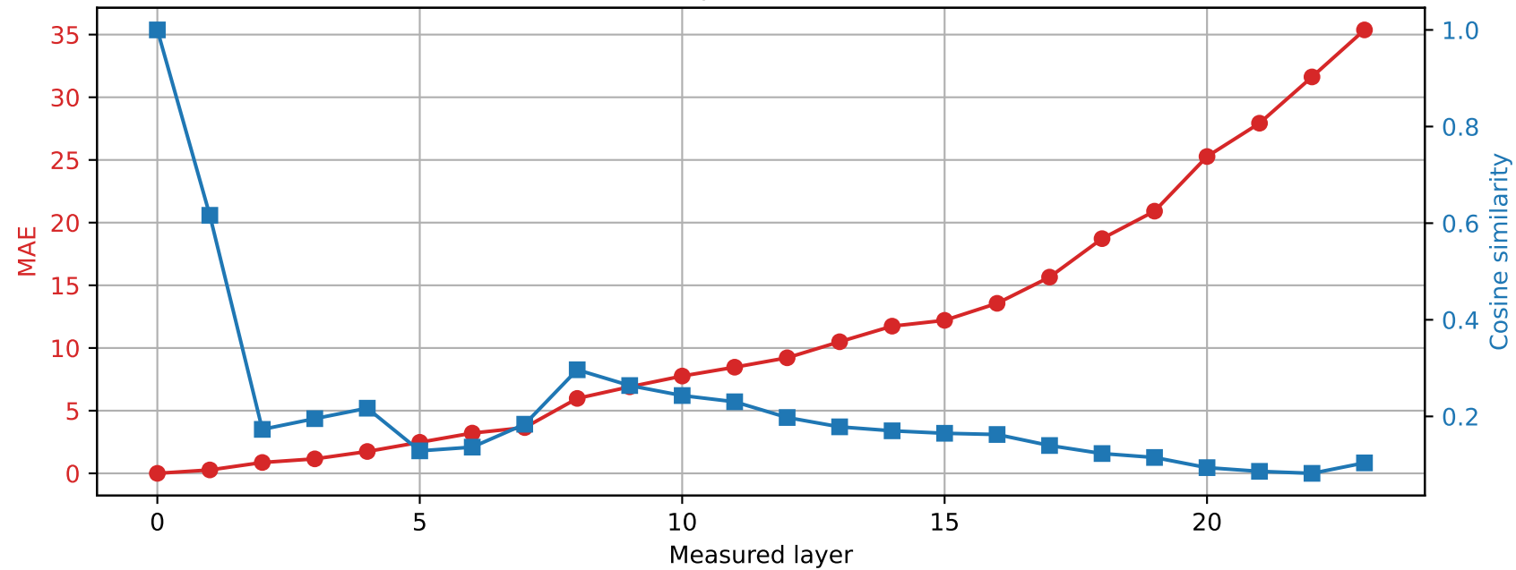
SmolLM2-1.7B-Instruct | Prompt 2 Spared layer 5 | Hybrid vs unquantized
