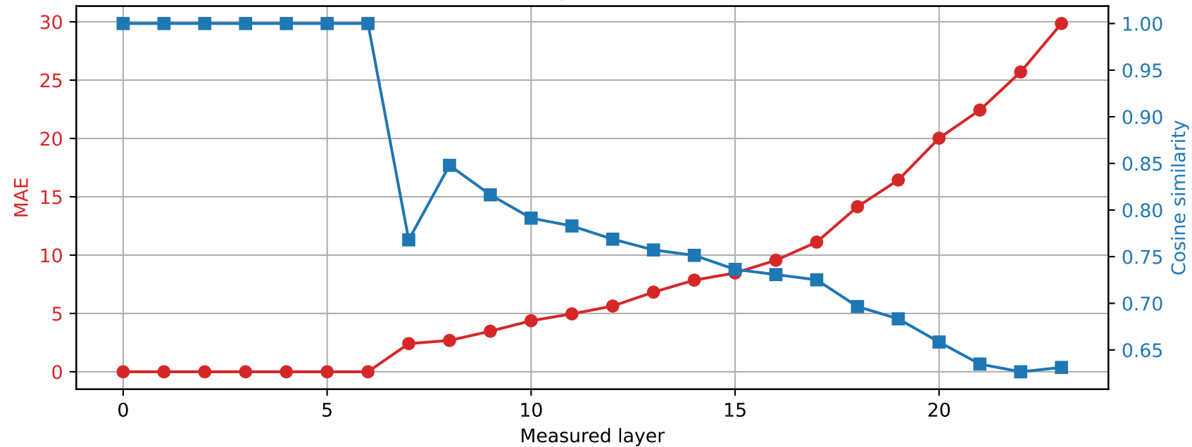
SmolLM2-1.7B-Instruct | Prompt 2 Spared layer 6 | Hybrid vs quantized
