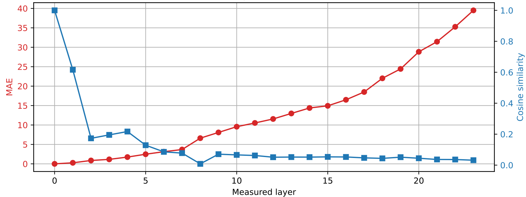
SmolLM2-1.7B-Instruct | Prompt 2 Spared layer 7 | Hybrid vs unquantized
