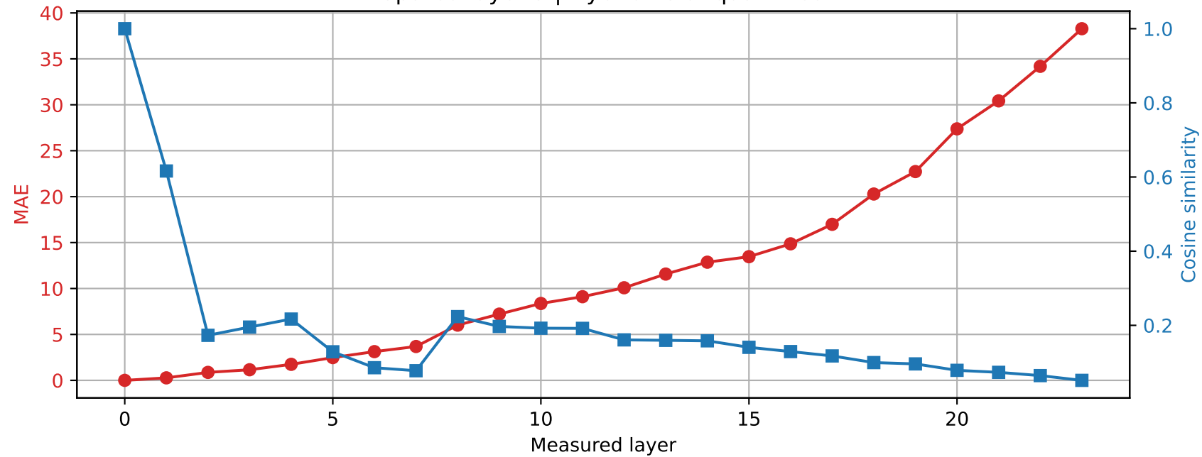
SmolLM2-1.7B-Instruct | Prompt 2 Spared layer 9 | Hybrid vs unquantized
