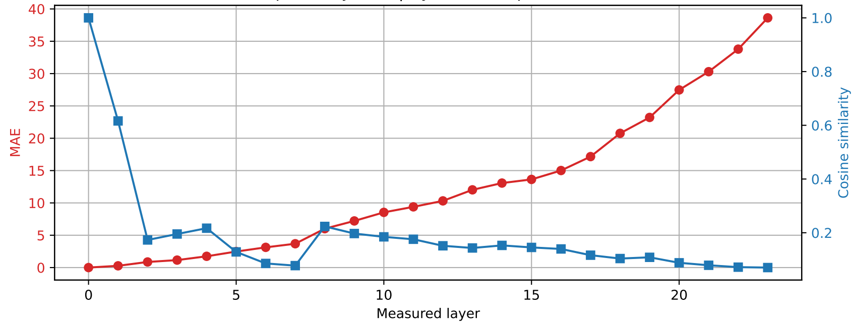
SmolLM2-1.7B-Instruct | Prompt 2 Spared layer 13 | Hybrid vs unquantized
